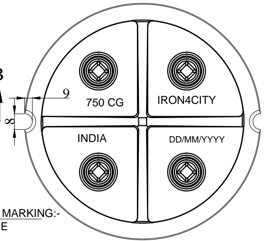
COVER BOTTOM VIEW
